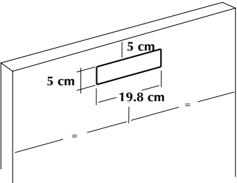
Touch handle WX1 maniglia Touch WX1 poignée Touch WX1 tirador Touch WX1
